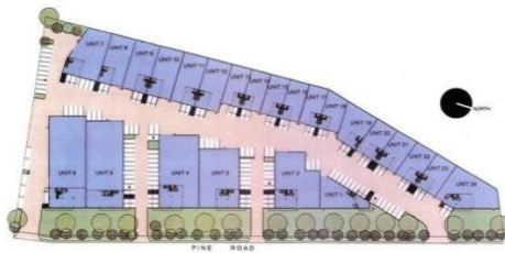
SITE/ GROUND FLOOR PLAN SCALE: 1:10 000 AT 04 PROPOSED DEVELOPMENT AT LOTS 1, 2, 3, 11 - DP 205712 AND DP 231327 PINE ROAD, YENNORA
